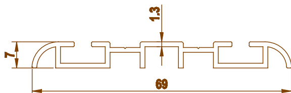
3709 0.440 kg/m
